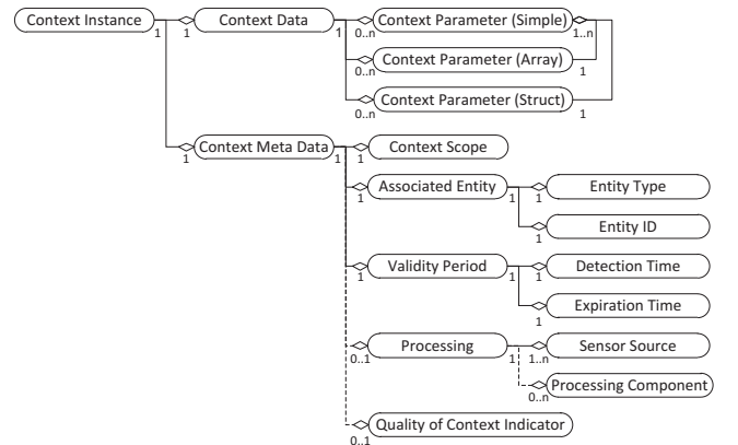
Fig. 7. Context meta data in the ContextML schema [30]
