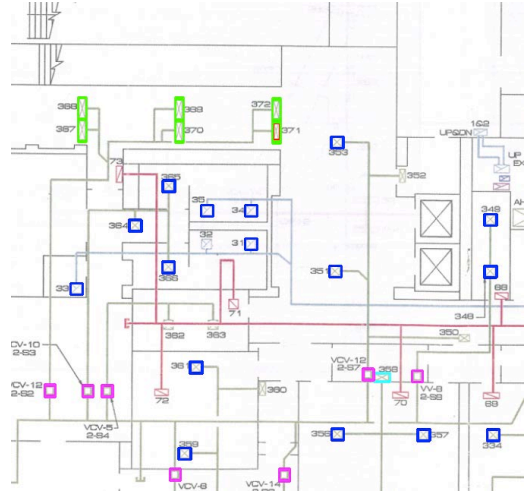
Figure 5. Example of parsing an image to identify air handlers, VAV boxes, and dampers
